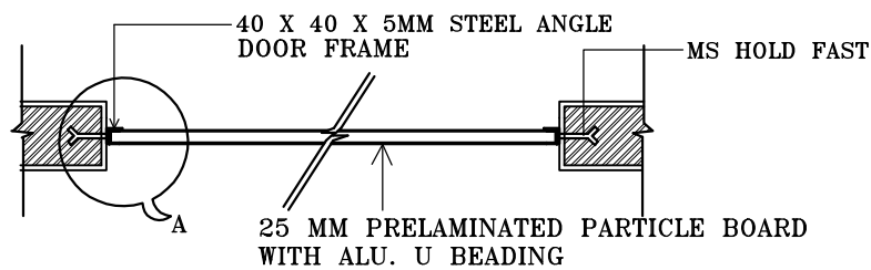
SECTION AT X'-X' N.T.S.
